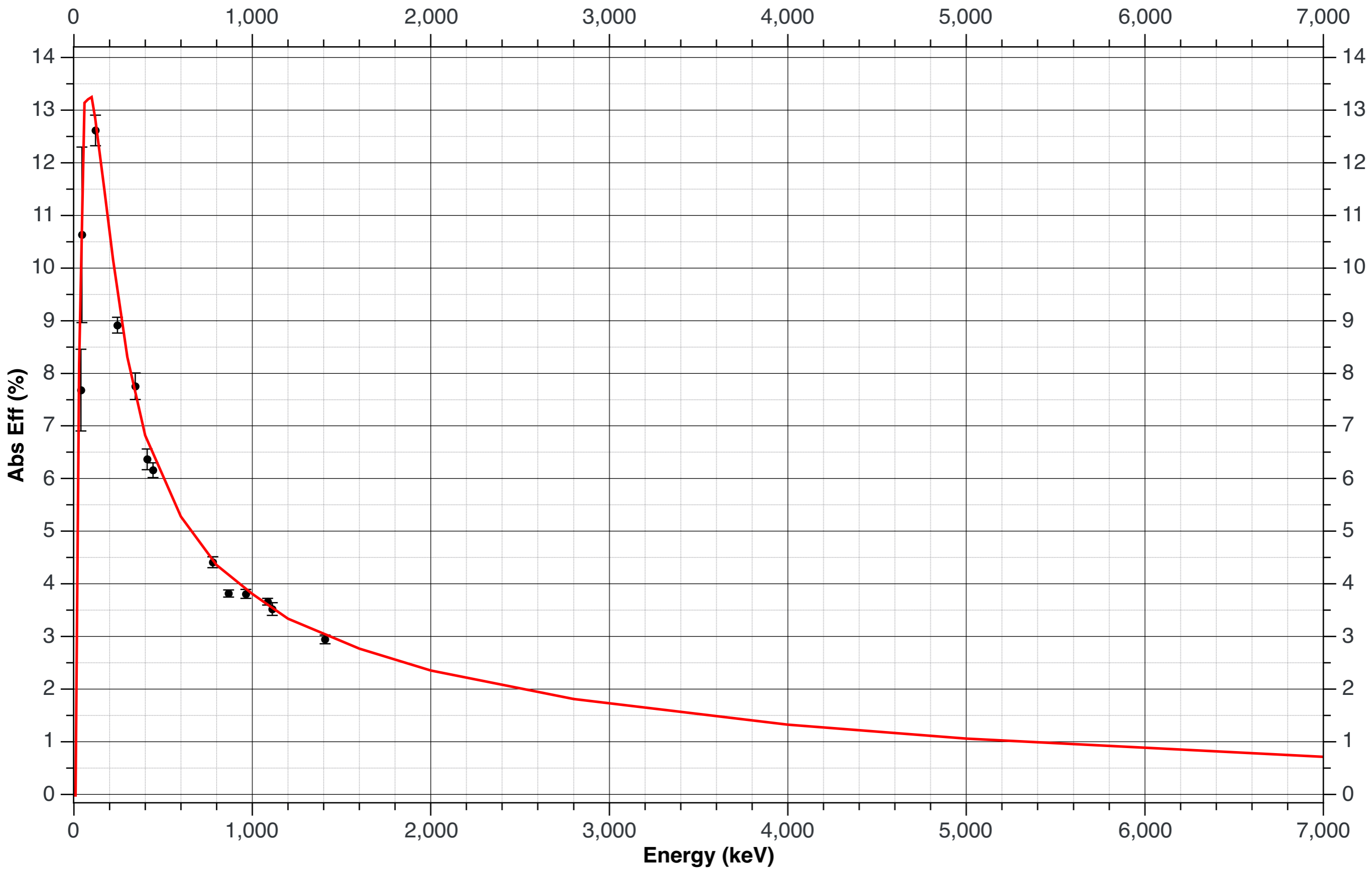
IS605 - 4 Clovers - addback (152Eu vs Geant4 (0.75))
