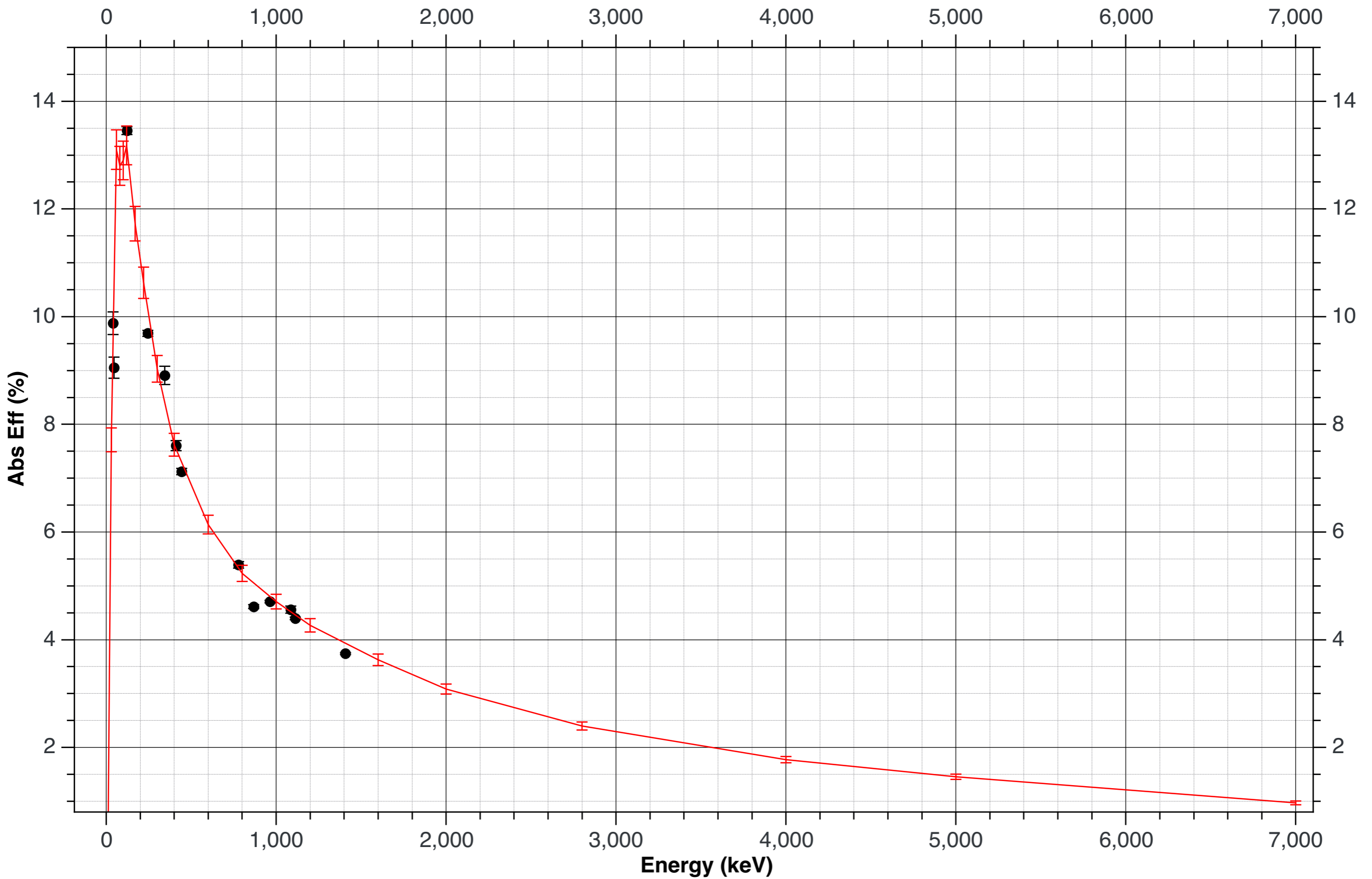
IS530 - 5 Clovers - addback (152Eu vs Geant4)
