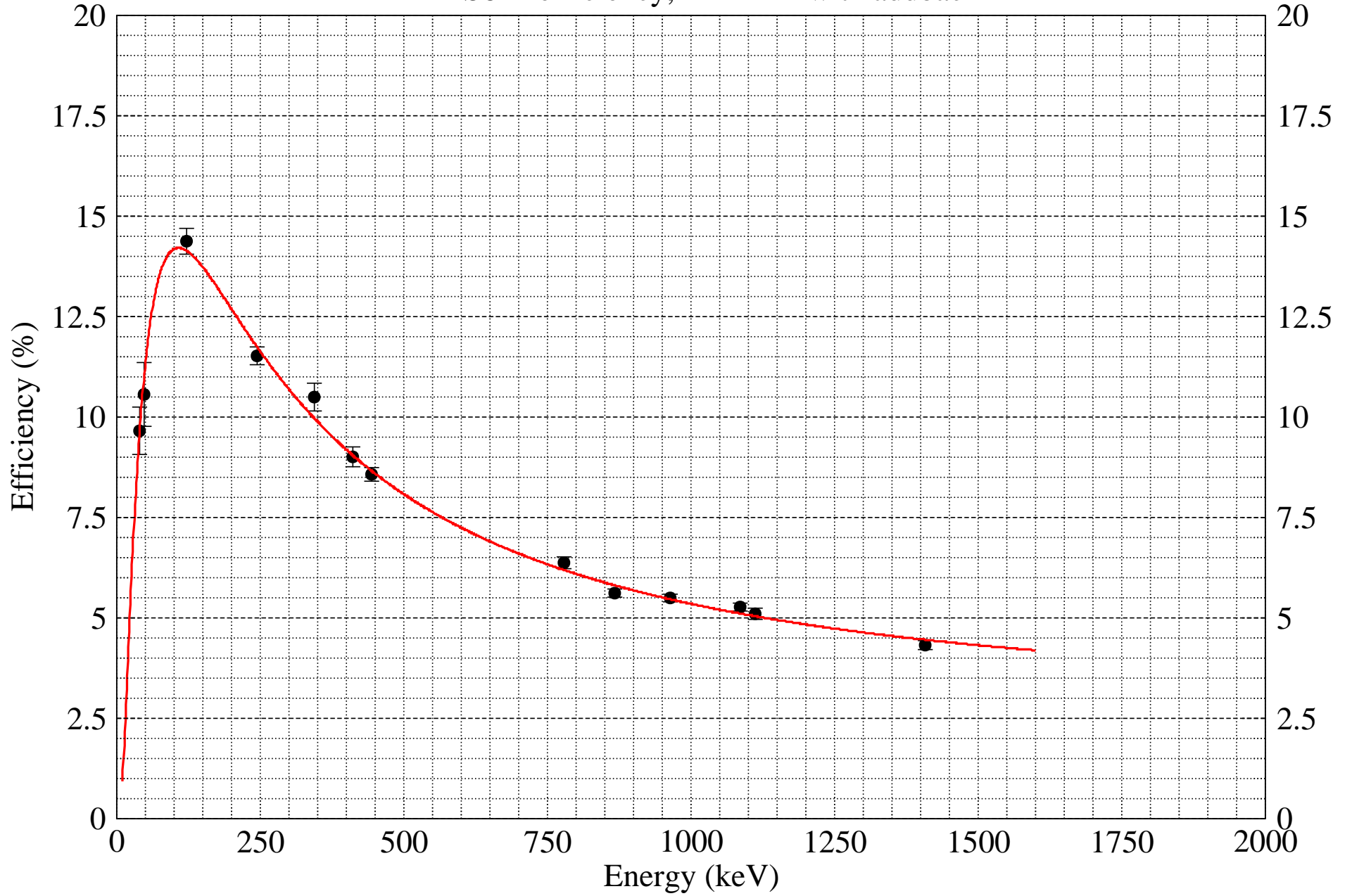
IS622 efficiency, 6 clovers with addback
